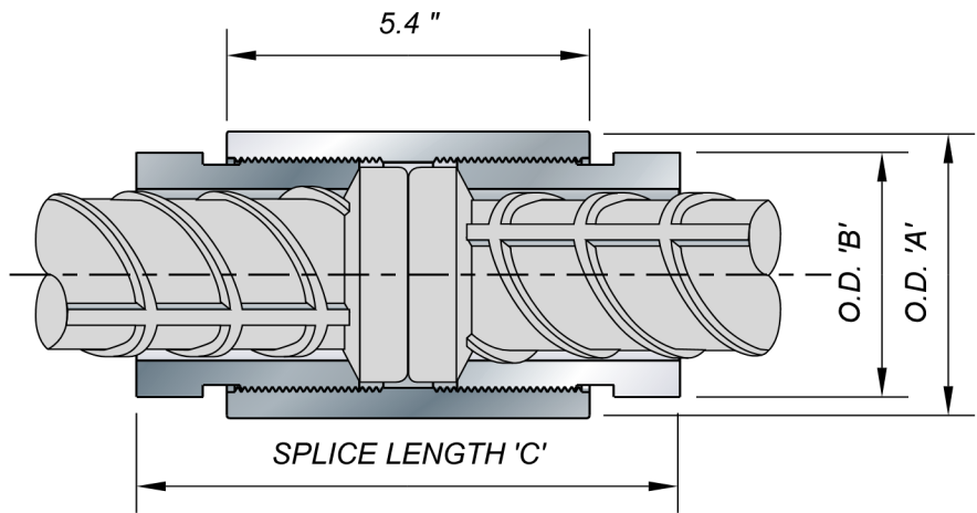
SECTION ALONG X-X
